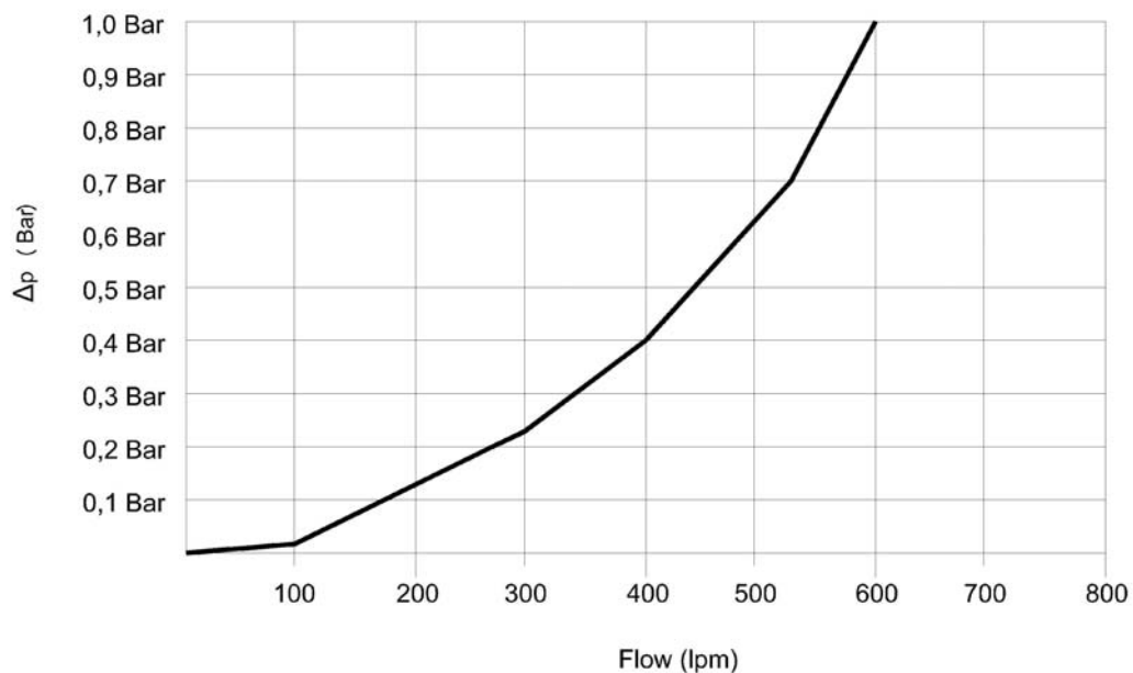
2 1/2" Mixer
