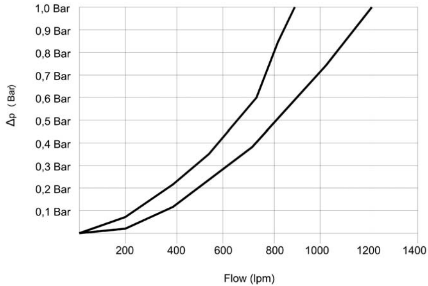
4" Mixer
