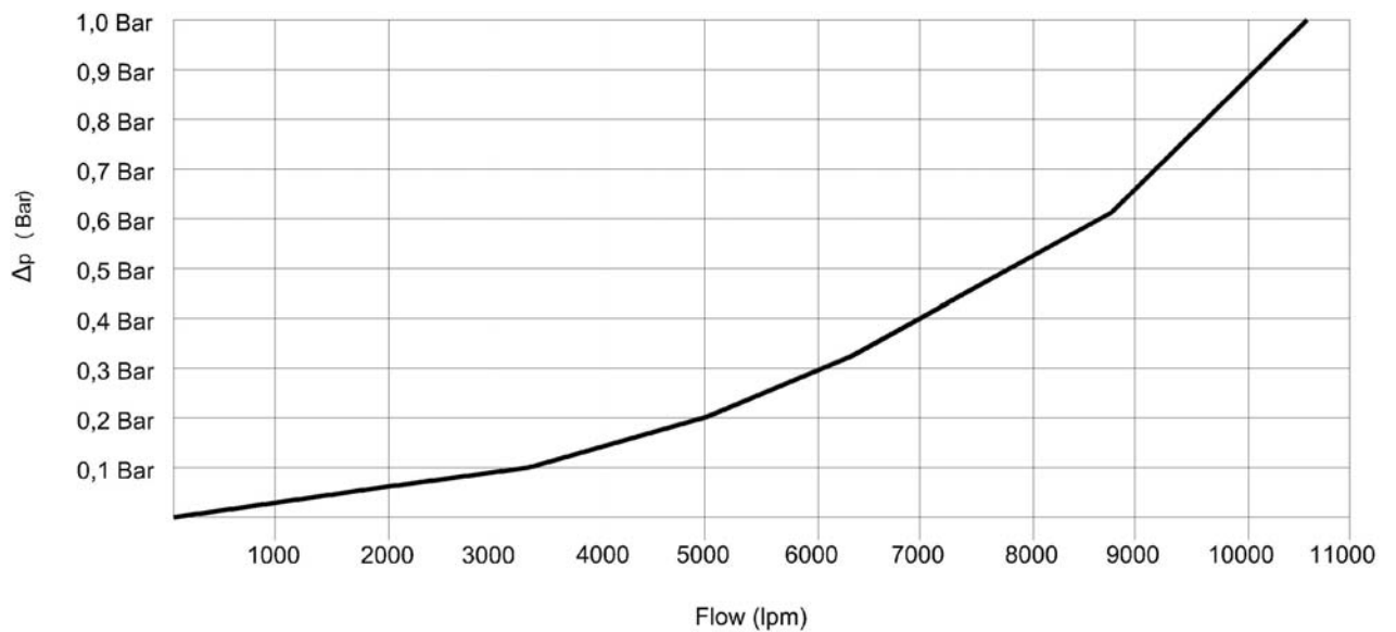
10" Mixer
