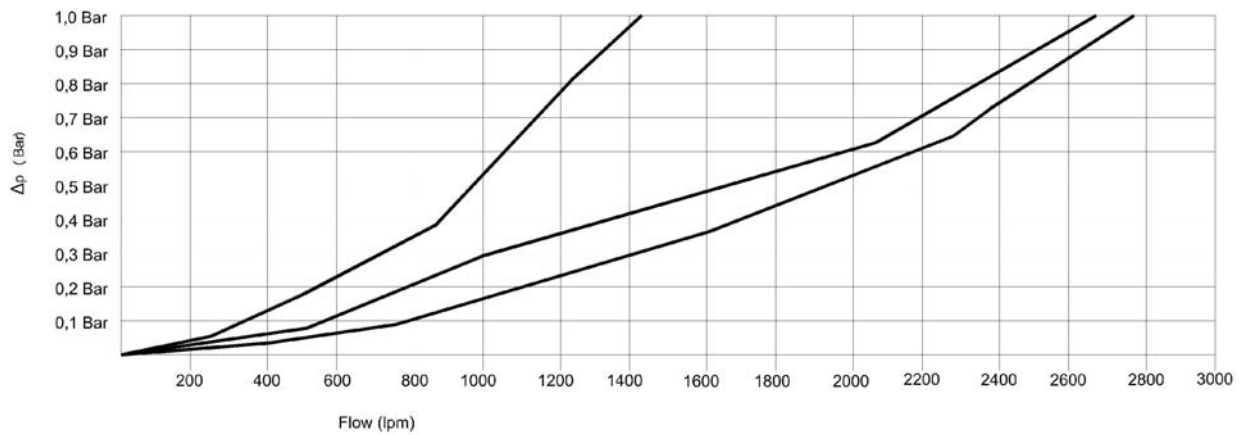
6" Mixer
