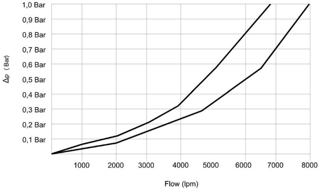
8" Mixer
